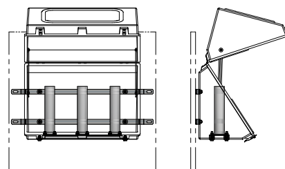
TYPICAL ASSEMBLY 387
