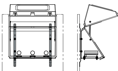
TYPICAL ASSEMBLY 287
