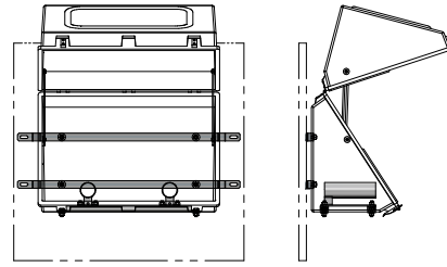
TYPICAL ASSEMBLY 357
