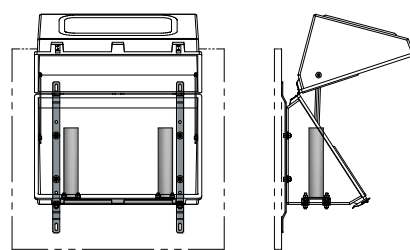
TYPICAL ASSEMBLY 297
