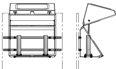
TYPICAL ASSEMBLY 377
