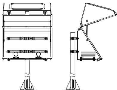
TYPICAL ASSEMBLY 157
