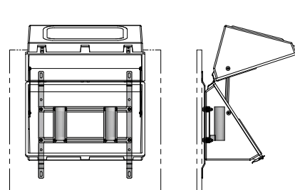
TYPICAL ASSEMBLY 177
