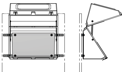
TYPICAL ASSEMBLY 397
