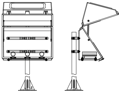
TYPICAL ASSEMBLY 167
