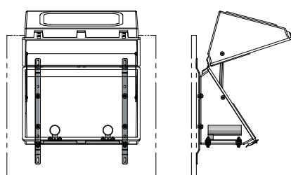
TYPICAL ASSEMBLY 277
