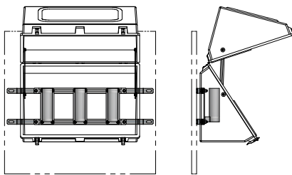
TYPICAL ASSEMBLY 347
