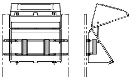
TYPICAL ASSEMBLY 337
